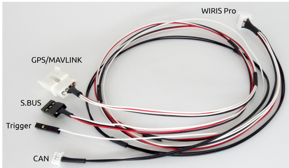
Figure 3 – WIRIS Pro interface cable pinout.
